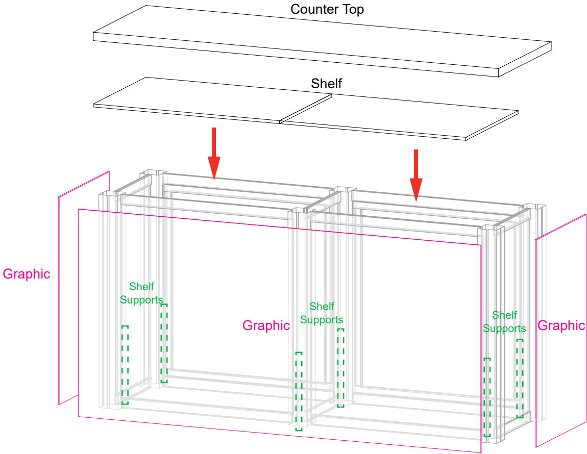
FRONT VIEW
