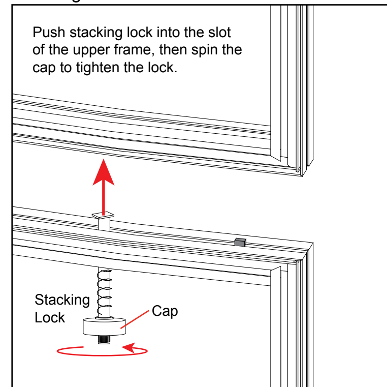
Stacking
